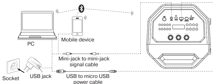
Fig. 2. Connection diagram
