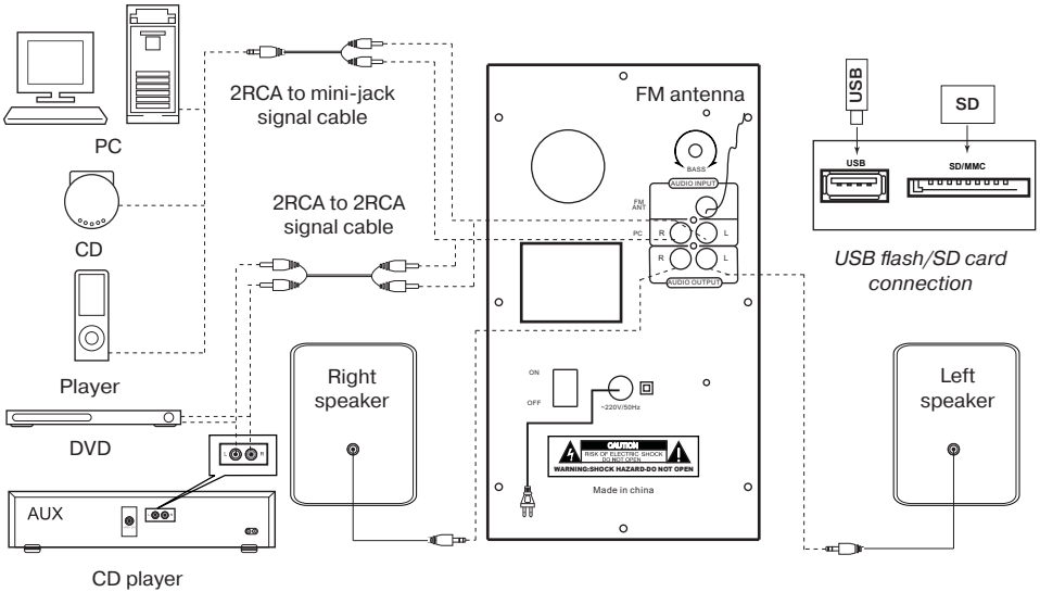
Fig. 4. Connection diagram
