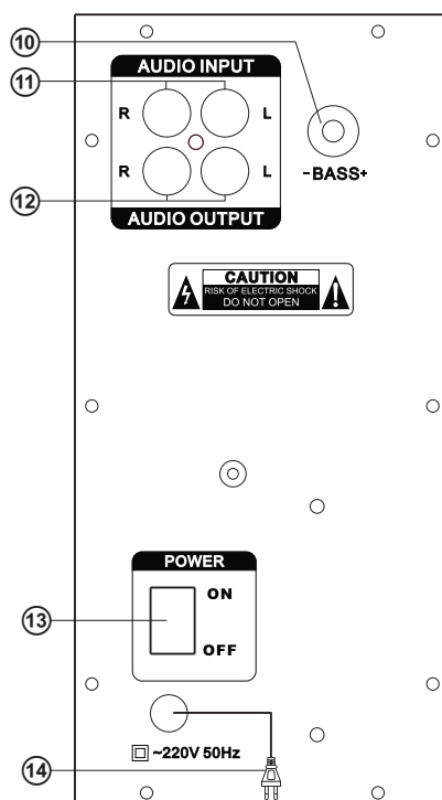
Fig. 2. Rear panel
