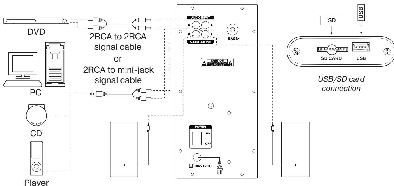
Fig. 5. Connection diagram
