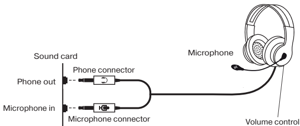
Fig. 1. Connection diagram
