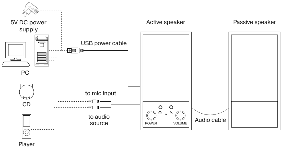
Fig. 2. Connection diagram
