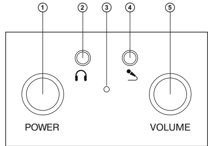
Fig. 1. Control panel
