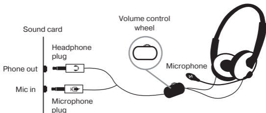
Fig. 1. Connection diagram
