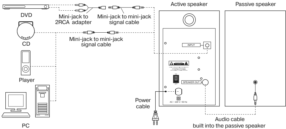
Fig. 3. Connection diagram
