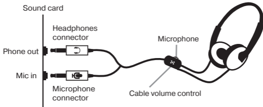
Fig. 1. Connection diagram
