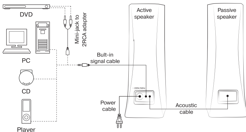
Fig. 2. Connection diagram
