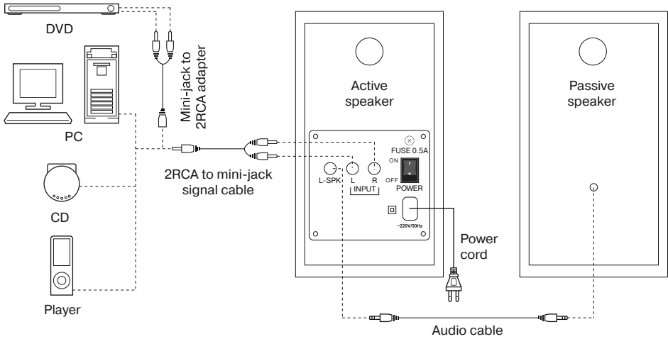
Fig. 2. Connection diagram
