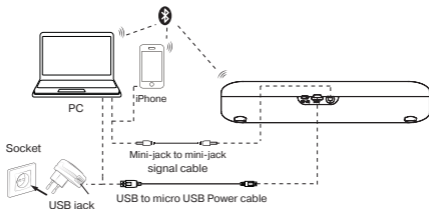
Fig. 2. Connection diagram
