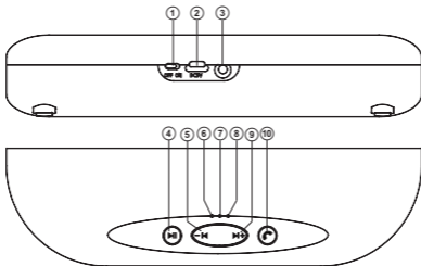
Fig. 1. Speaker system description
