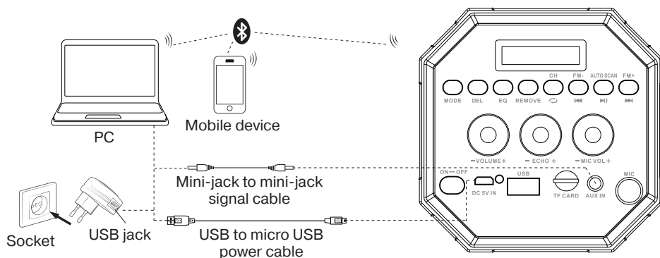
Fig. 2. Connection diagram
