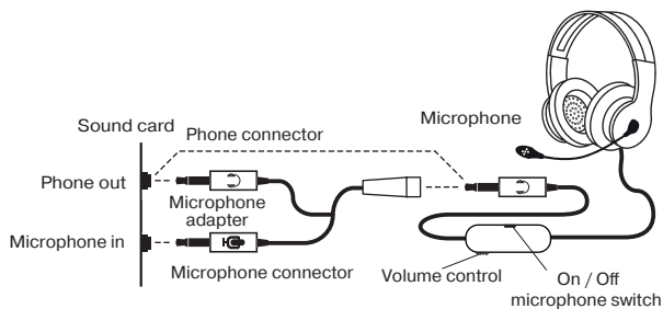
Fig. 1. Connection diagram
