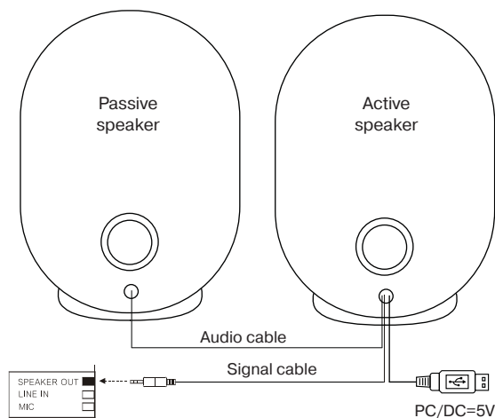
Fig. 2. Connection diagram
